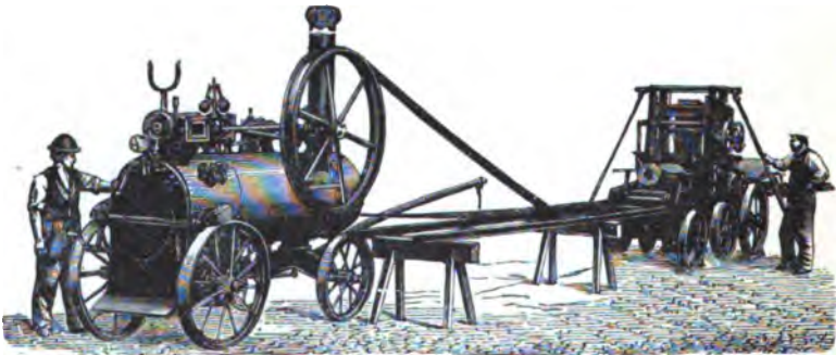
Fig. 303.—Transportable sawmill.
